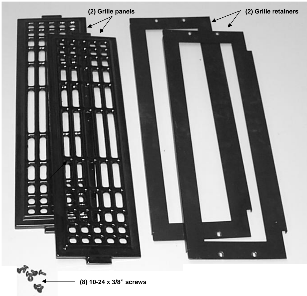
Figure 2 - Grille Components
